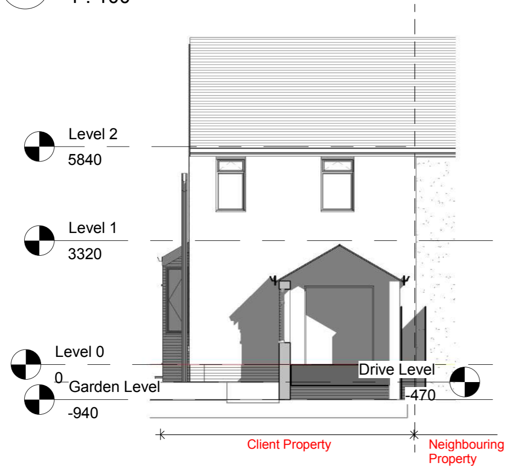
2 Short Section 1 : 100
